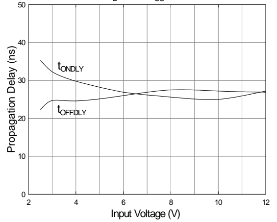
Fig. 18 Propagation Delay vs. Input Voltage C_L=15nF V_{CC}=15V
